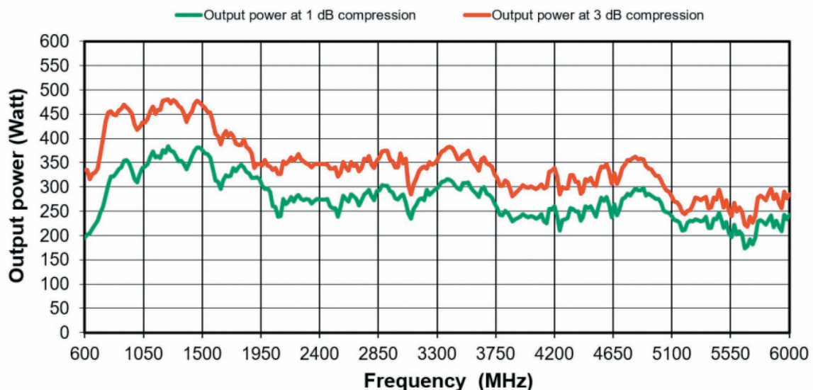
SX250 Typical Output
